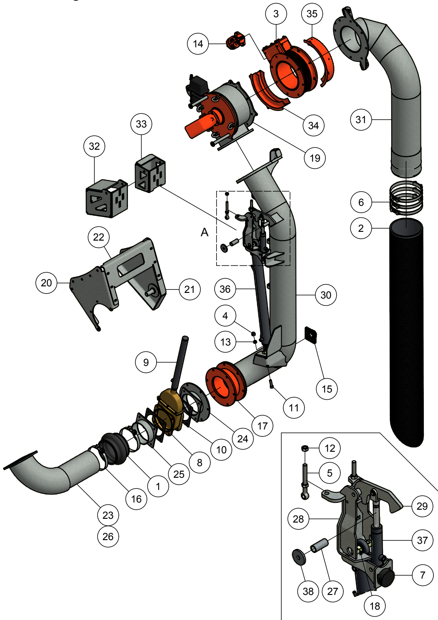
Detail A
